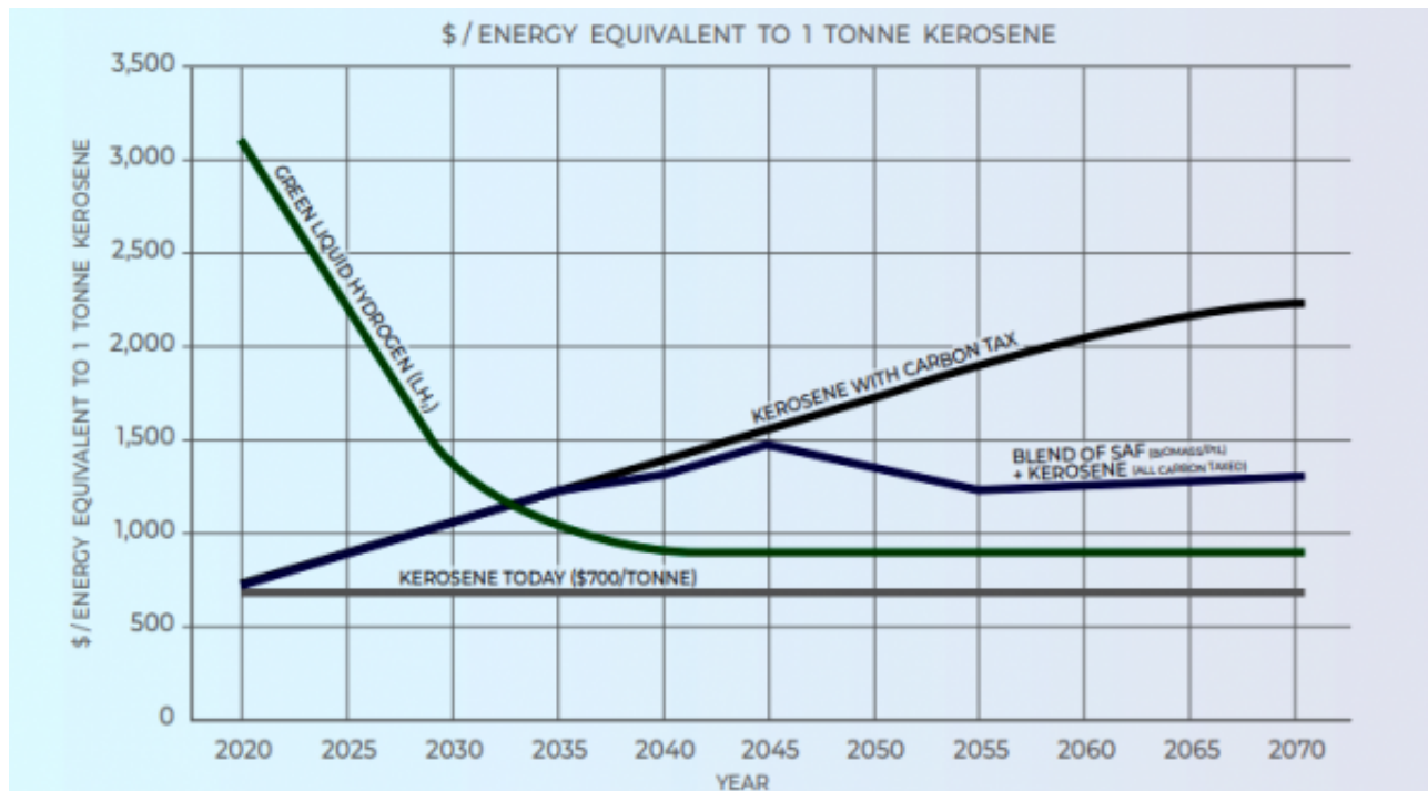
Figure 6 - Future cost of fuels (Source: FlyZero)
